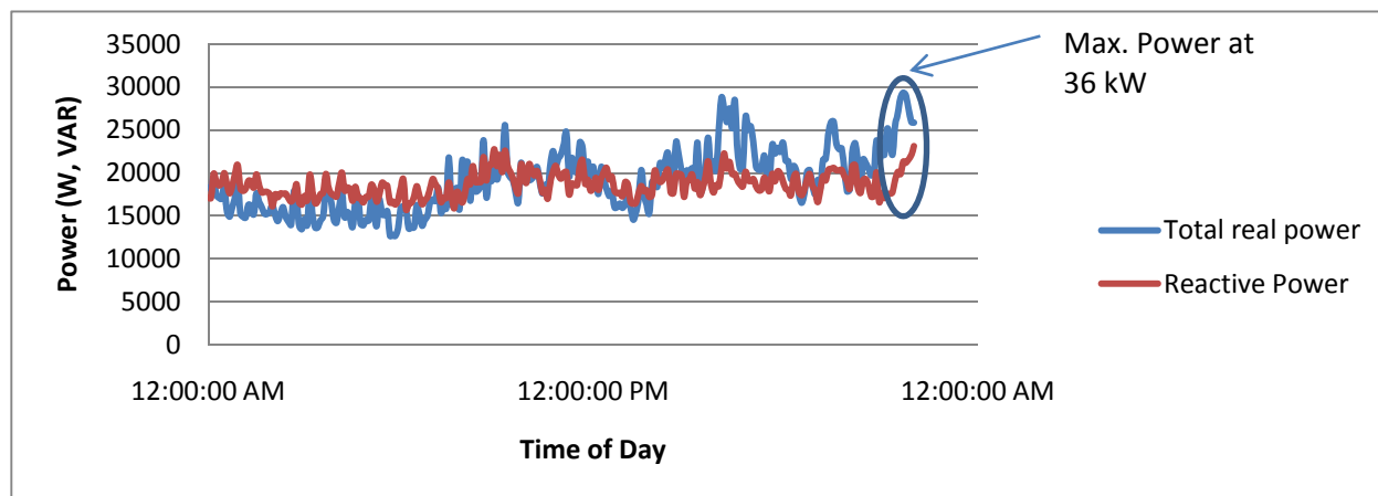
Figure 2. 9: Partial power demand profile up until the generator shut down at 9:45 p.m.
