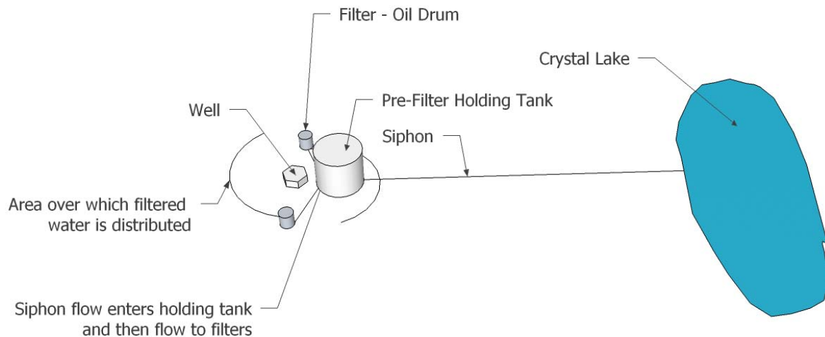
Figure 3.15: Diagram of possible set up with a pre-filter holding tank
