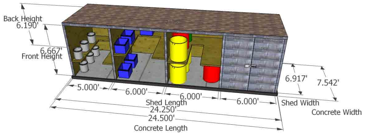
Figure 7.6: Dimensioned drawing of proposed design
