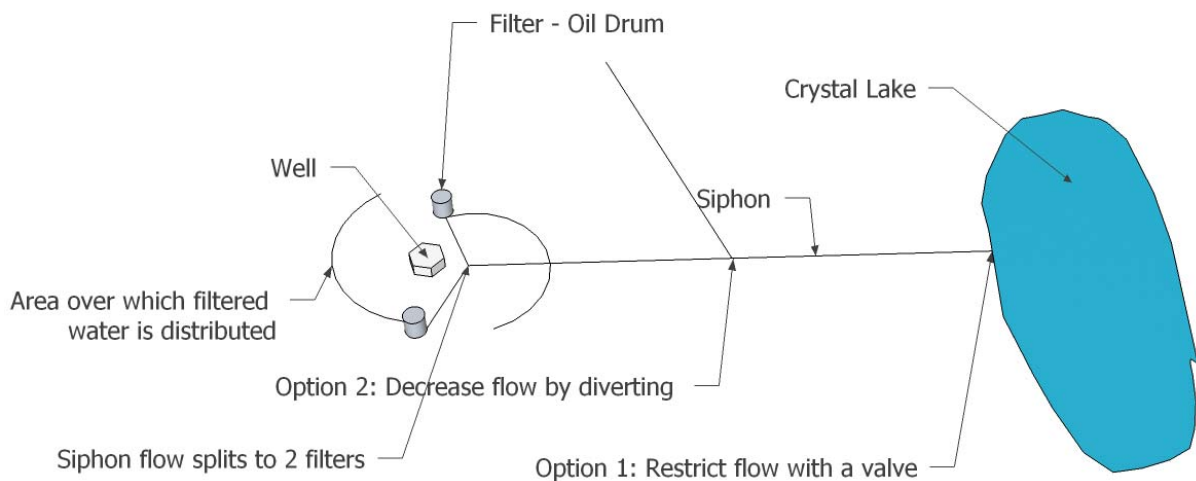
Figure 3.13: Diagram of a possible set up with the two drums.
