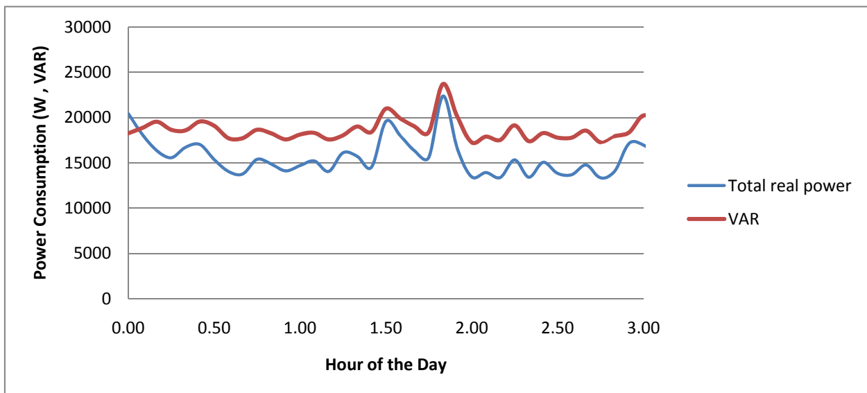
Figure 2.11: Large load that consumed both real and reactive power upon energizing.
