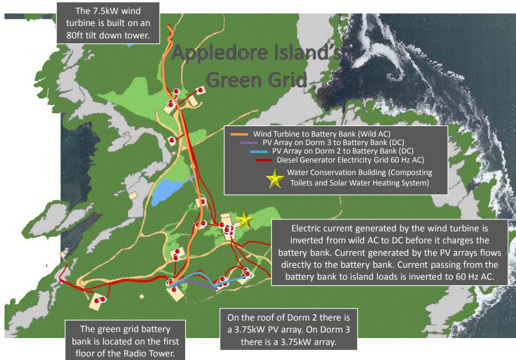
Figure 5.4: Diagram outlining the general details of SML's green grid.
