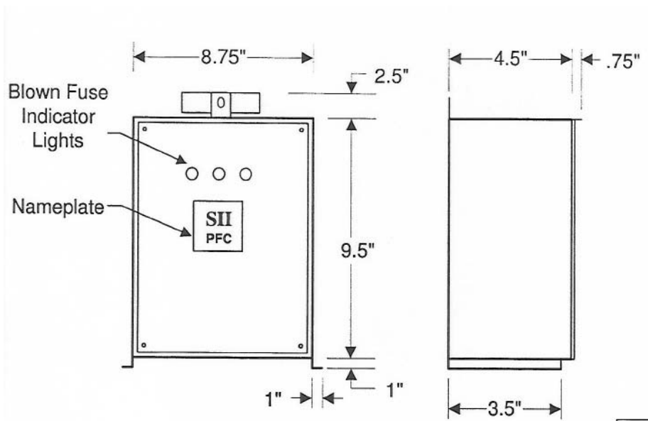
Figure 2.14: Dimensional information provided by Steelman Industries, Inc.
