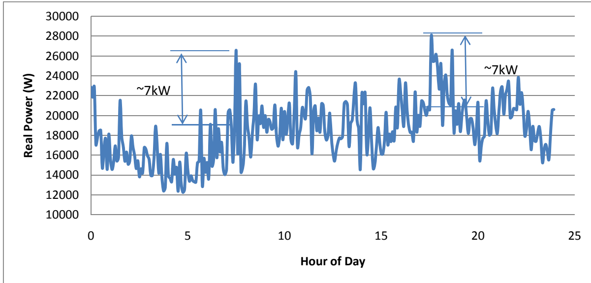
Figure 2.7: Power profile for June 16, 2011.
