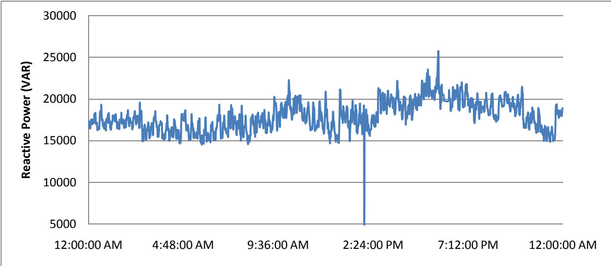
Figure 2.4: Reactive power profile for July 26, 2010
