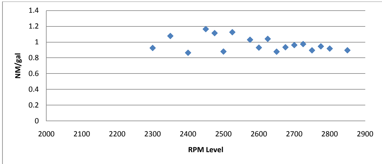
Figure 4.2: NM/gal for All Trips
