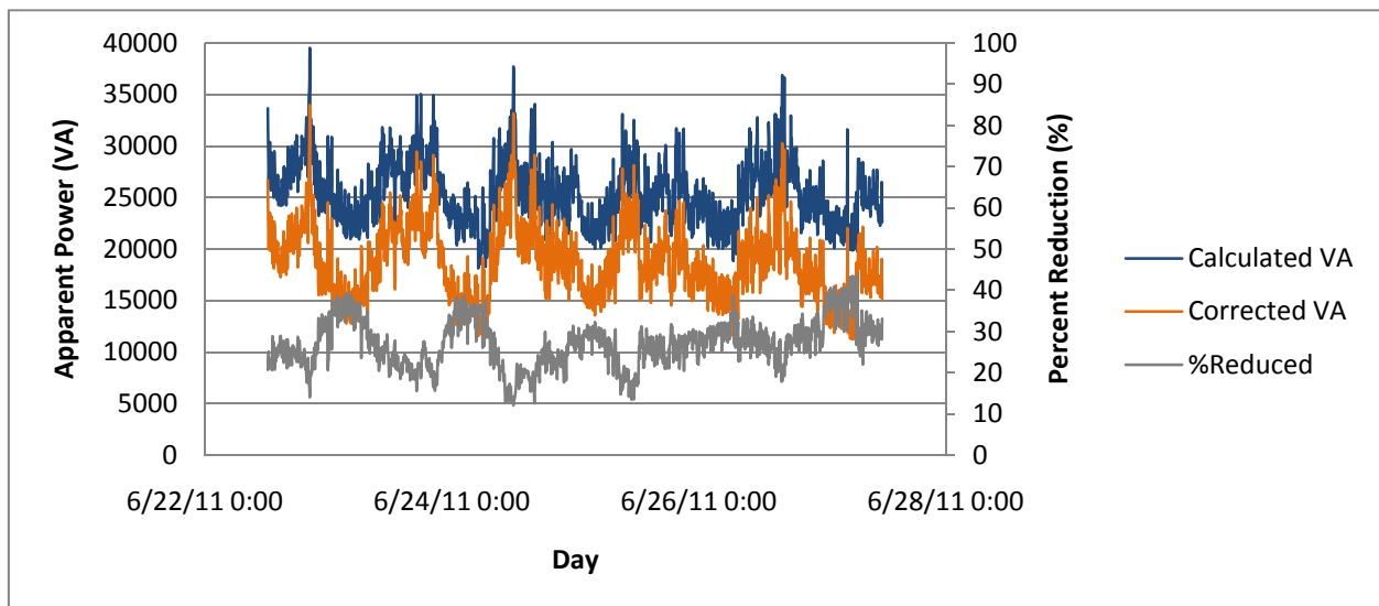
Figure 2.12: Measured apparent power, projected corrected apparent power, and percent reduction in apparent power for June 23 – 26, 2011.
