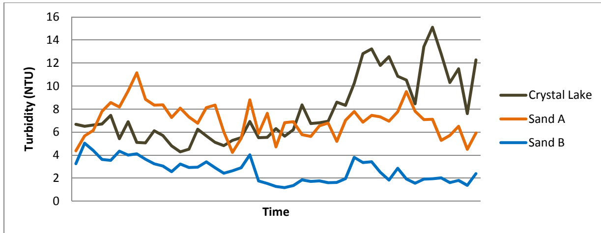
Figure 3.5: Turbidity results over the three week sampling period.
