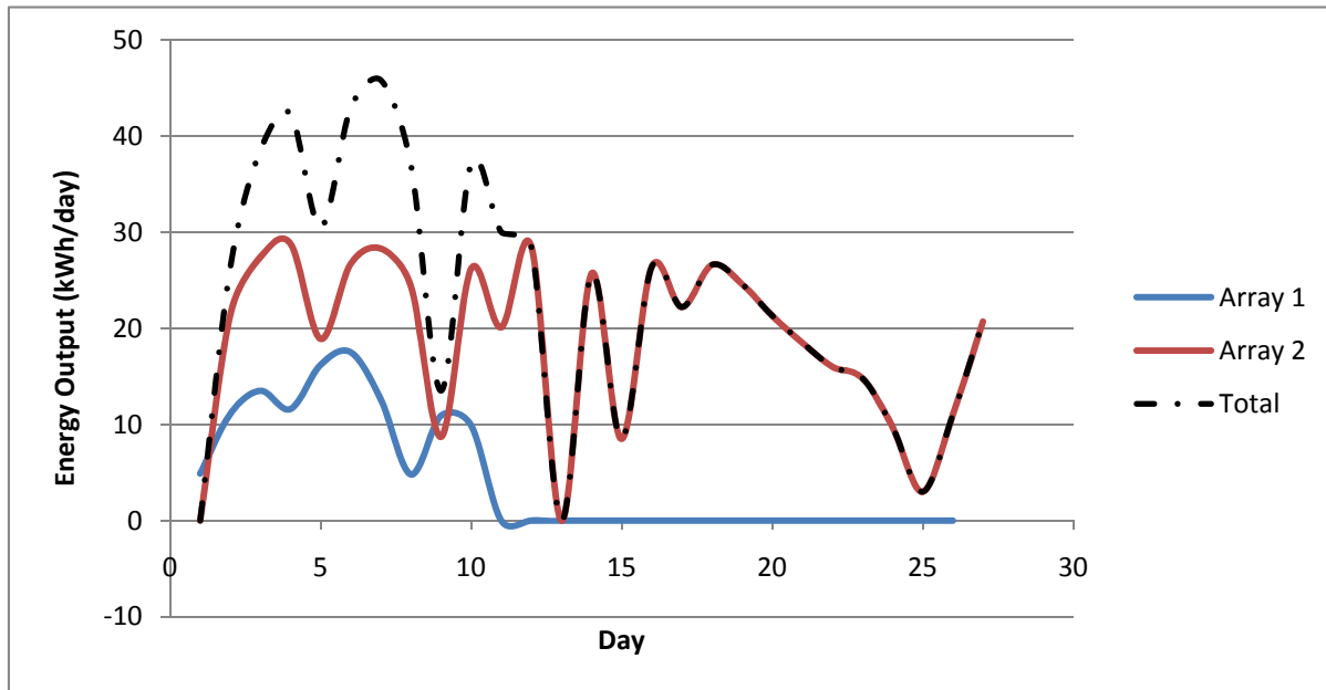
Figure 1.1: Output recorded by the OutBack charge controllers from August through September 2010.
