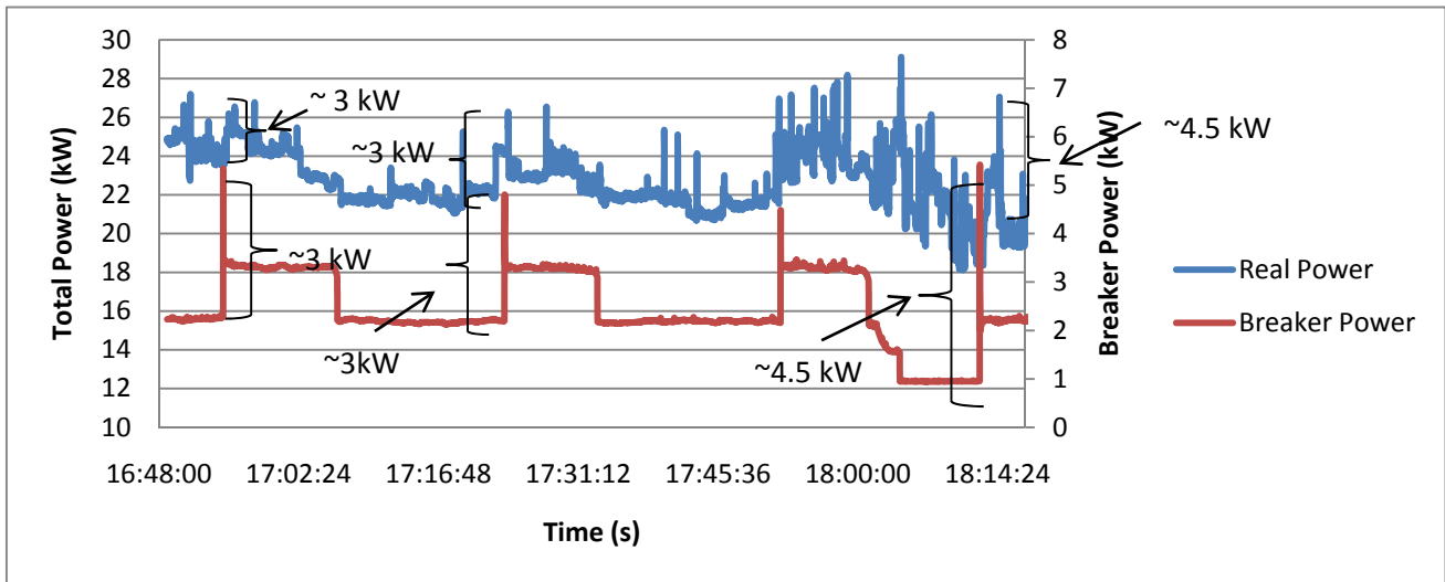
Figure 2.8: Simultaneous power monitoring of the entire grid as well as the circuit breaker for the refrigerator compressors.
