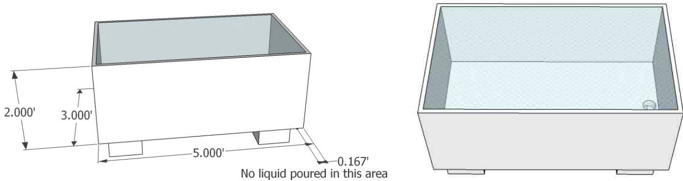
Figure 7.6: Proposed liquid compost design
