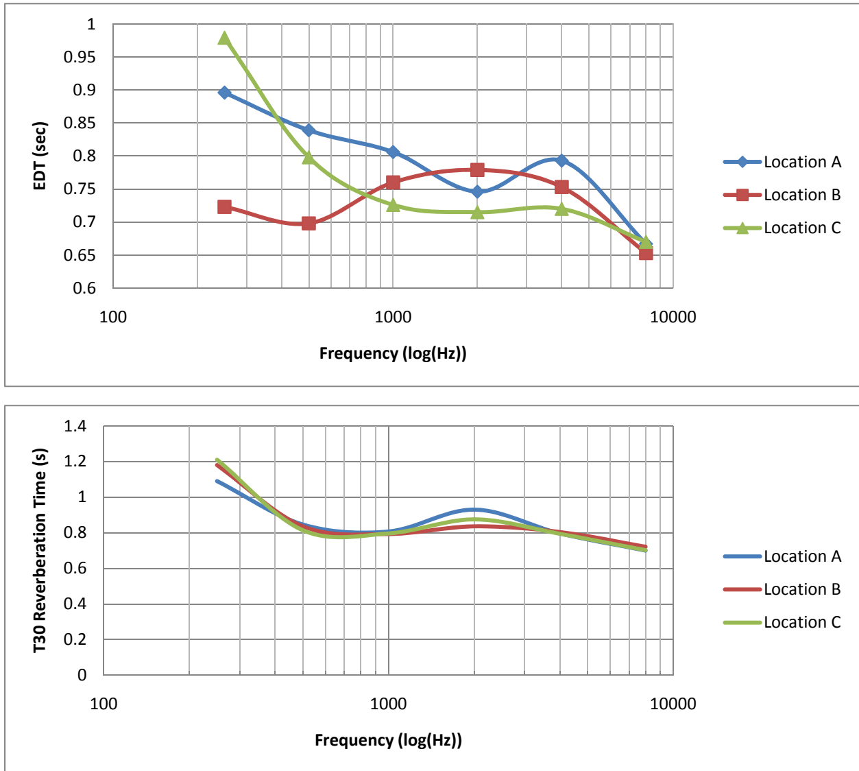
Figure 4.4: Calculated reverberation times from the T30 method and the EDT method shows a dependence of room positioning.
