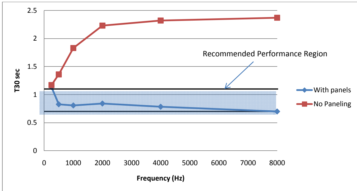
Figure 4.5: The effect that the Acoustic Paneling has on T30 calculated reverberation time as a function of frequency.
