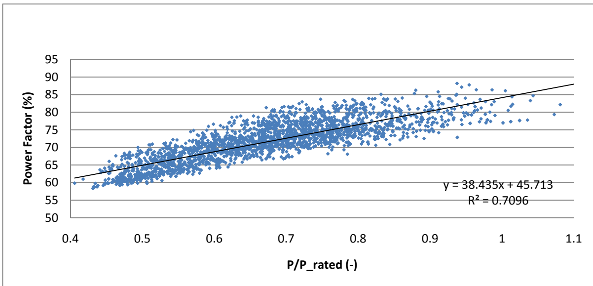
Figure 2.10: Power factor as a function of normalized power demand.
