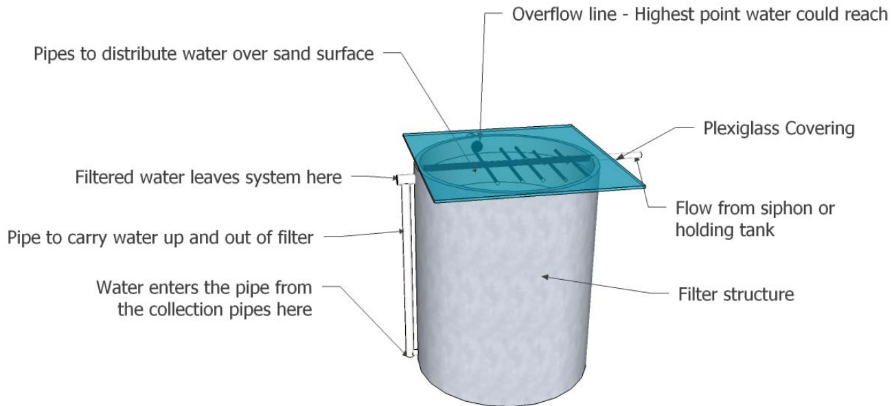
Figure 3.11: New filter design
