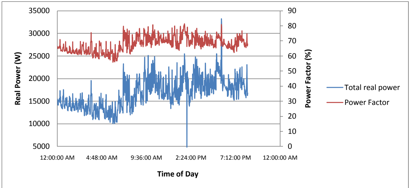
Figure 2.3: Power demand profile as well as the corresponding power factor for July 26, 2010. The generator shut down at approximately 5:40 p.m.
