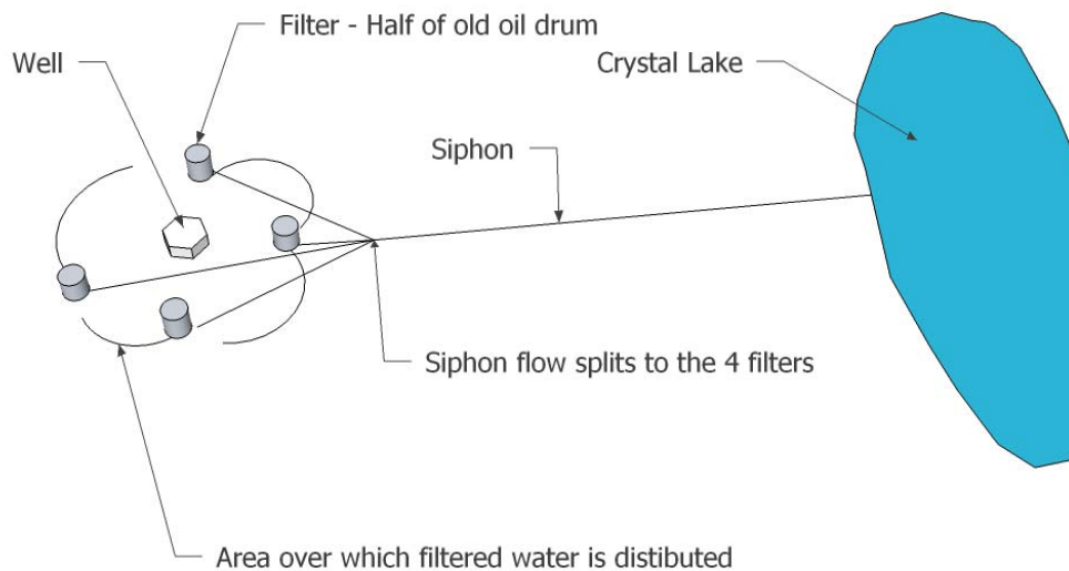
Figure 3.14: Diagram of a possible set up making 4 filters out of the drums.
